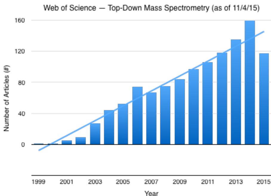
Figure. Sustained growth of top-down mass spectrometry as indicated by the number of articles published from 1999 to 2015 from Web of Science.
